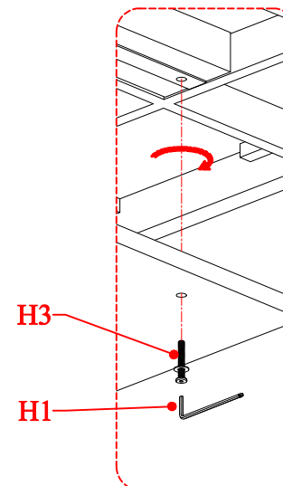
Detail 'B'
