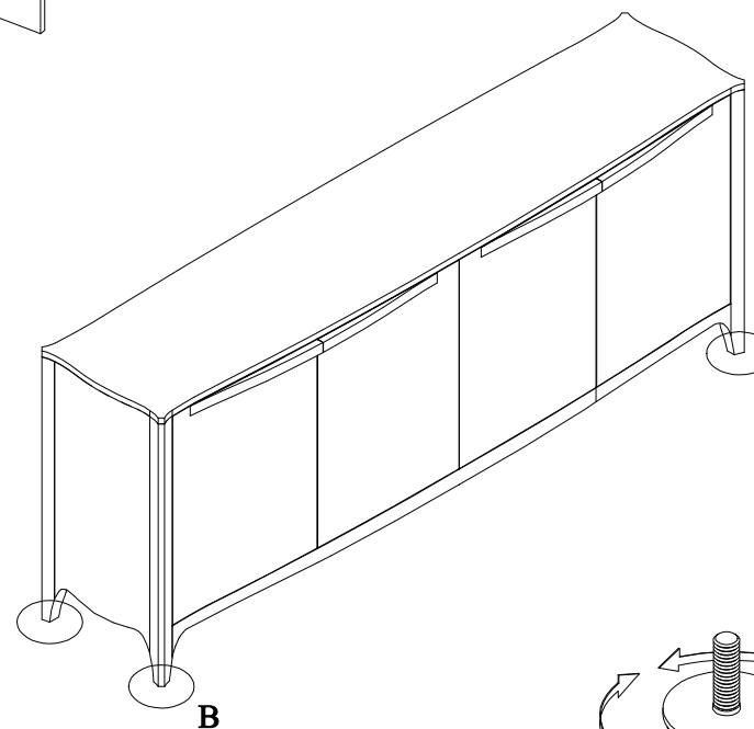
Detail 'B'
