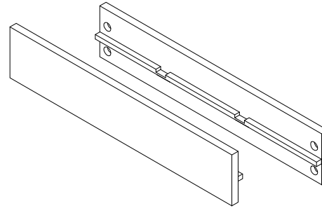
P3 Side rail (x 1)
