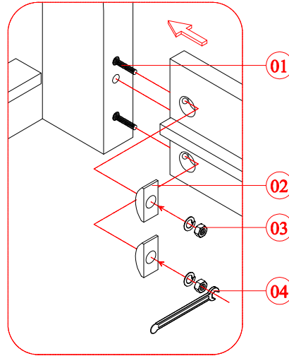
Detail 'B'
