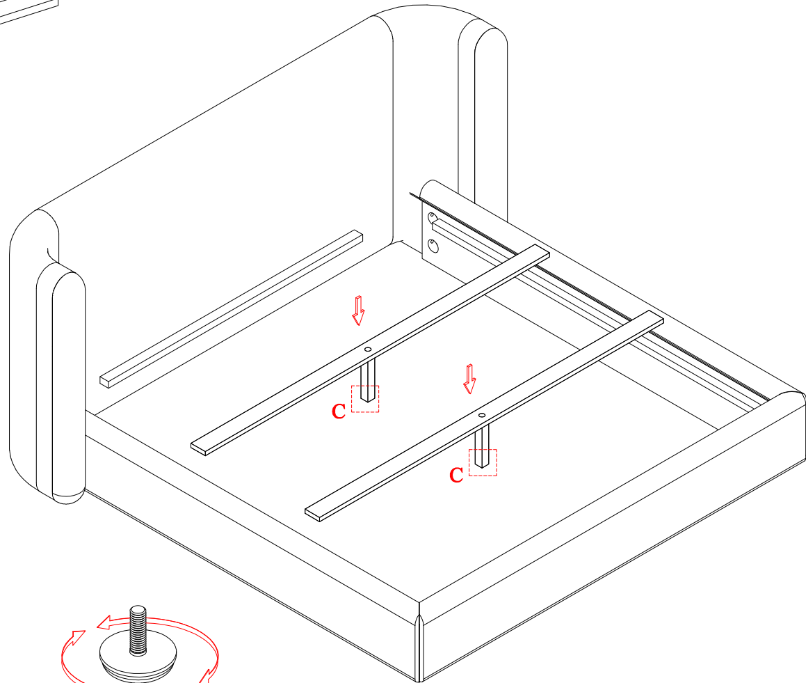
Detail 'C'
