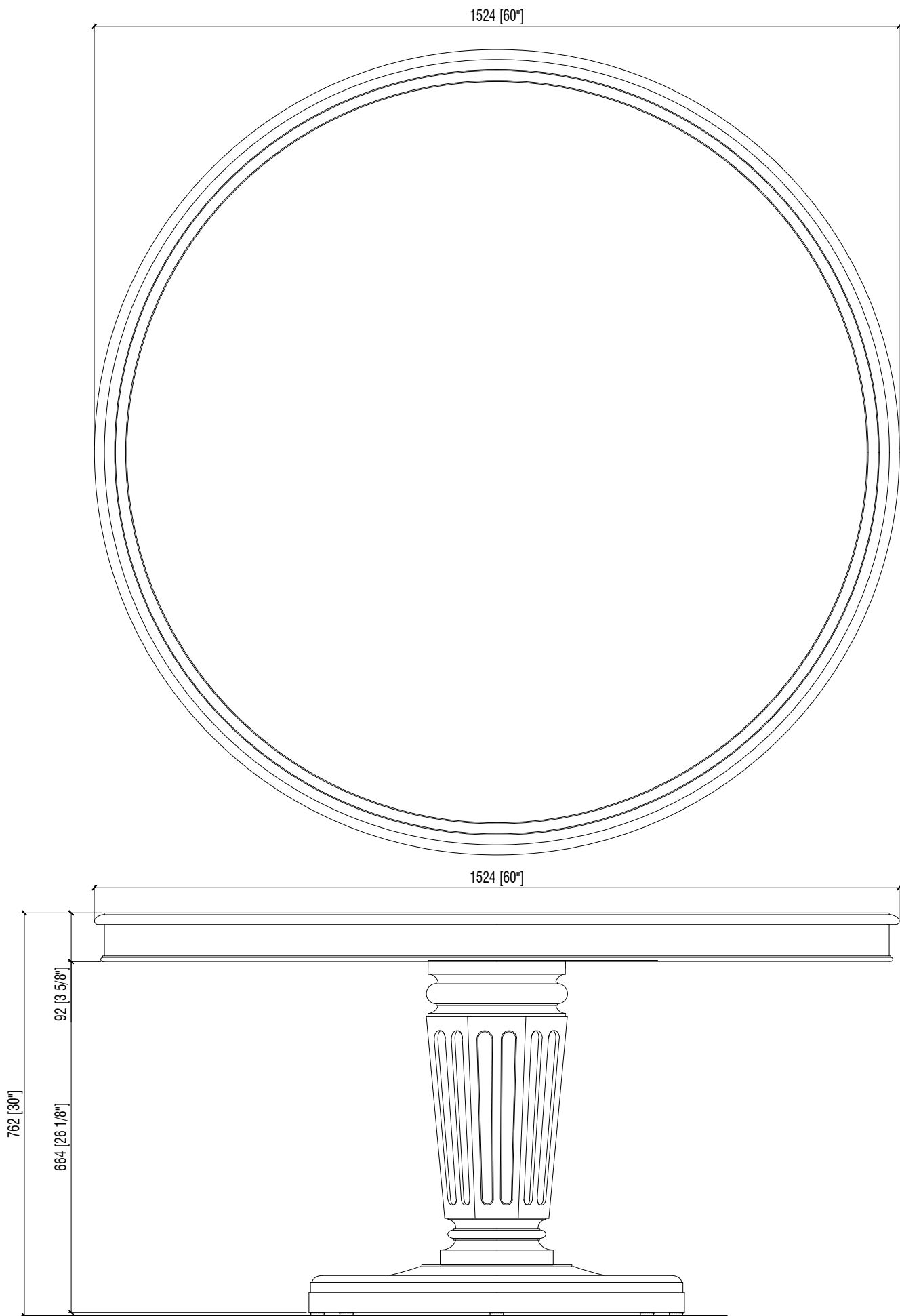
AL54066 ROUND DINING TABLE DIA 68 5/8" x 30" HT
