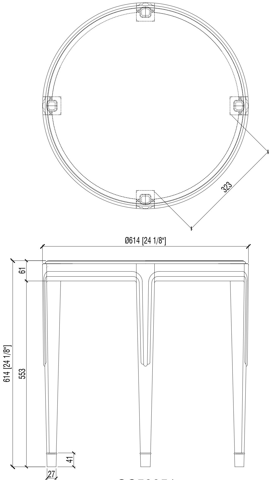
SC50051 DIA 24" x 24 1/8"HT Collection: DORCHESTER
