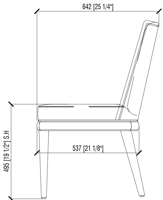
SIDE VIEW
