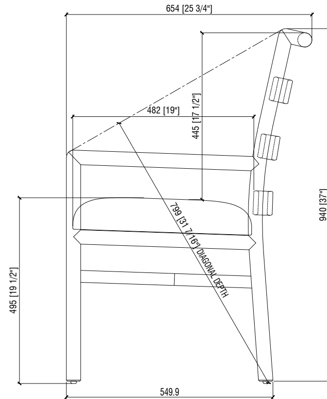
TA41082 DINING ARM CHAIR 23" x 25 3/4" x 37" HT
