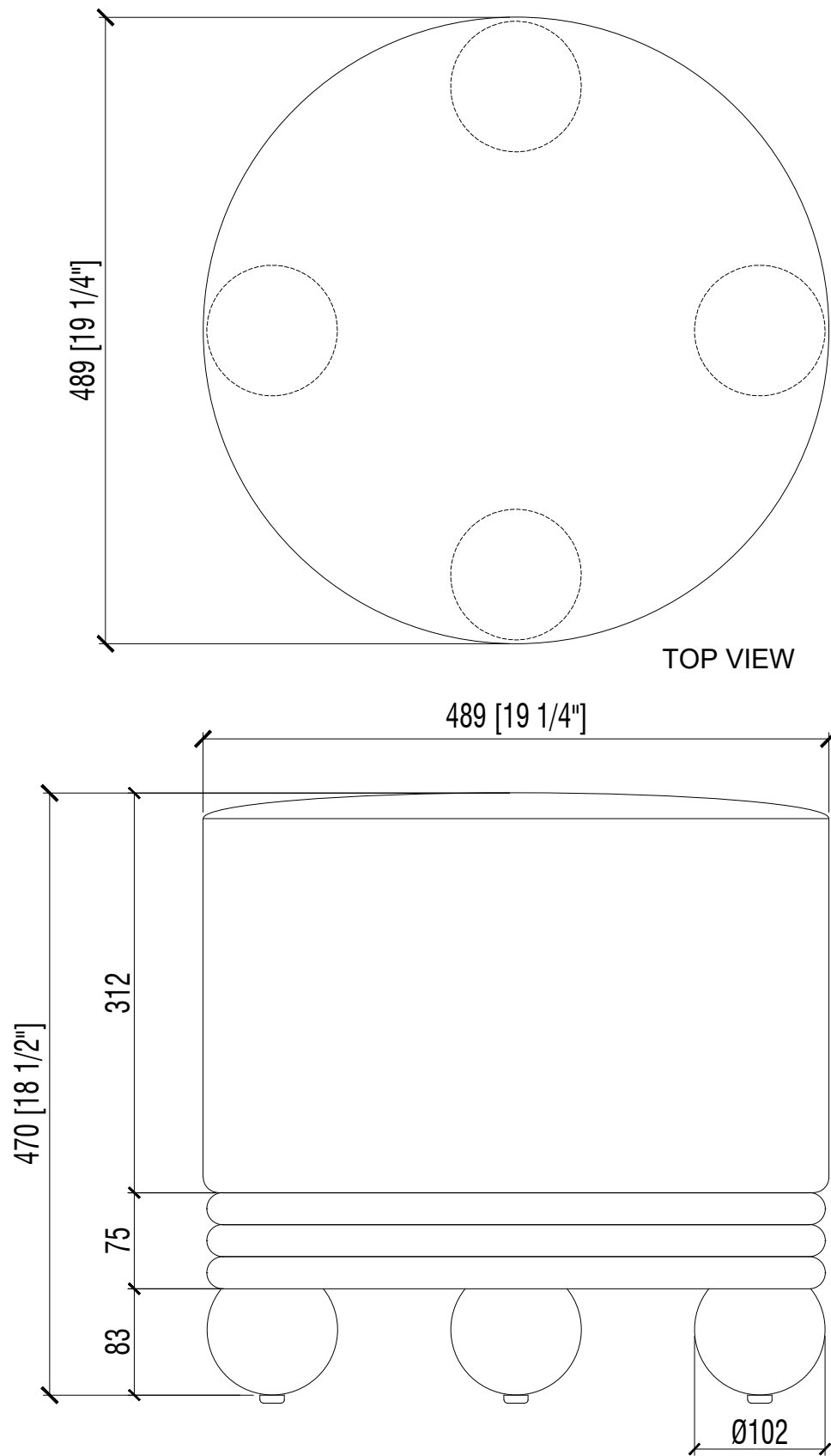
FRONT VIEW
