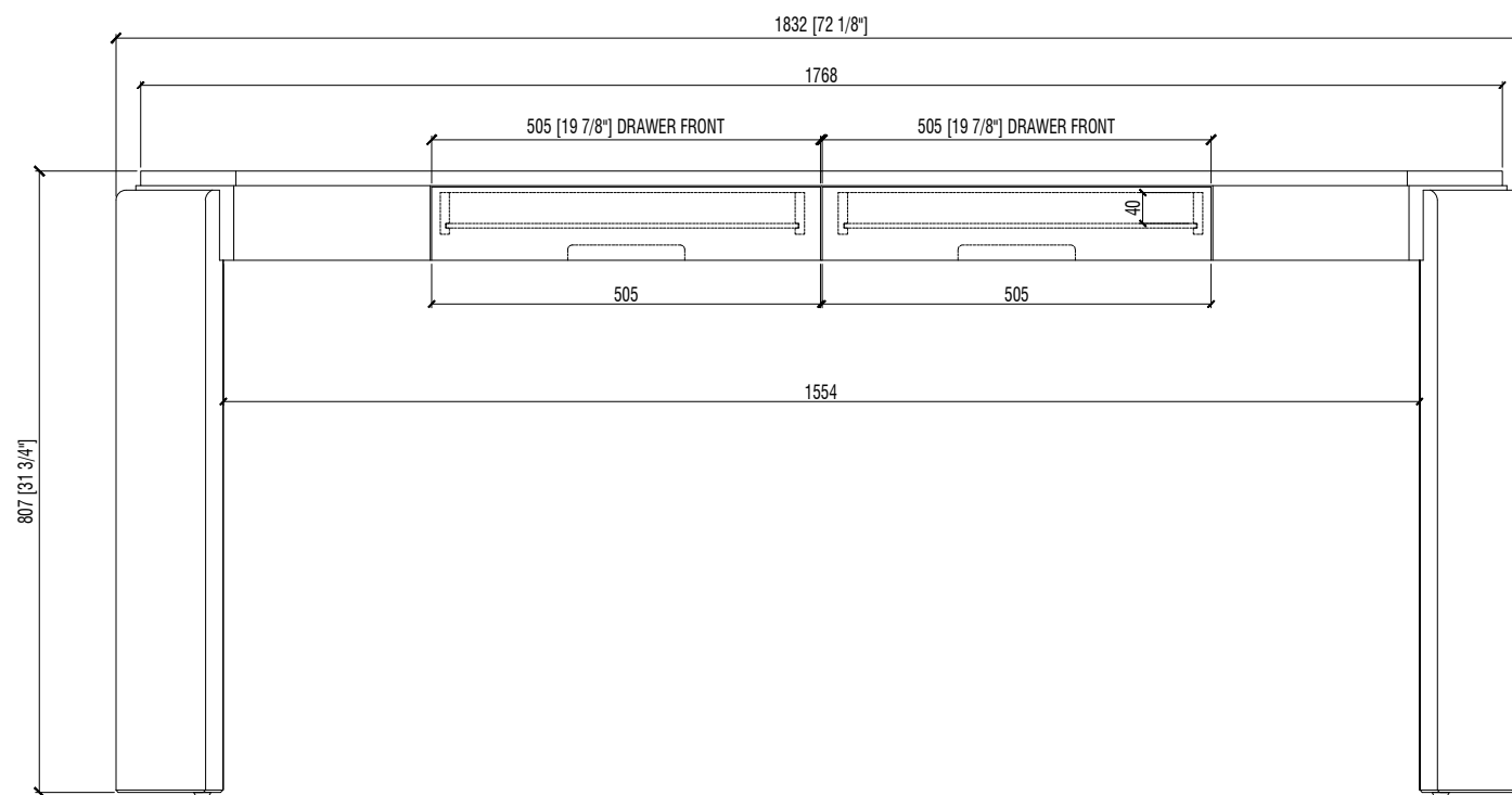
FRONT VIEW
