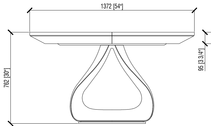
FRONT VIEW (CLOSE TABLE)
