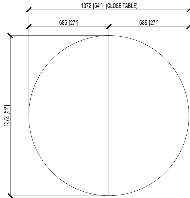
PLAN VIEW (CLOSE TABLE)
