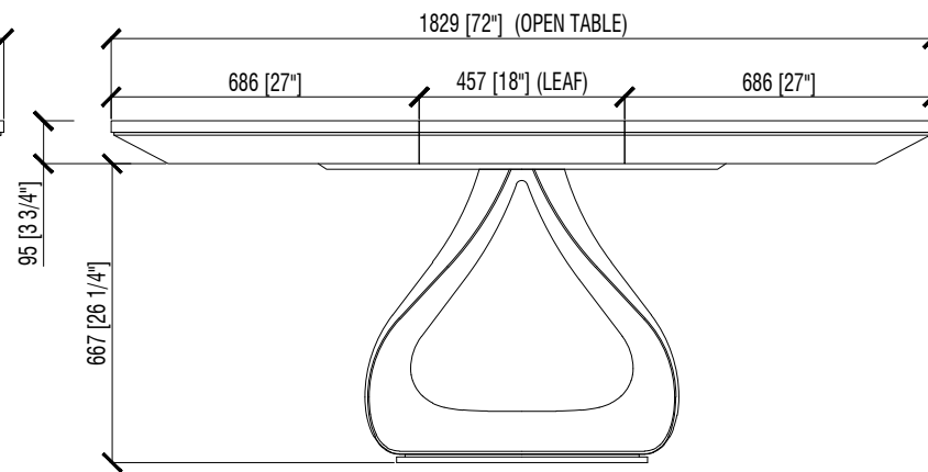
FRONT VIEW (OPEN TABLE)
