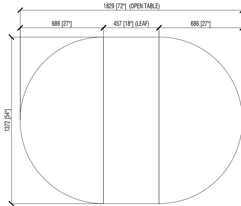
PLAN VIEW (OPEN TABLE)
