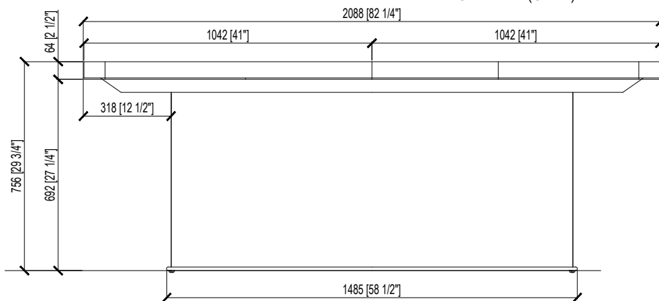
FRONT VIEW (CLOSE)
