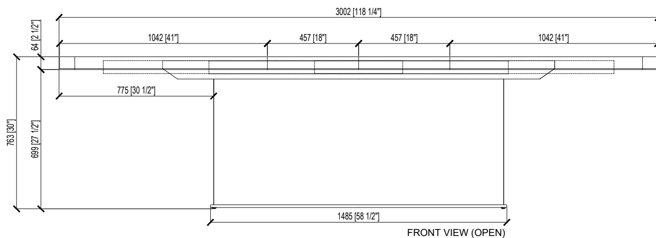
FRONT VIEW (OPEN)
