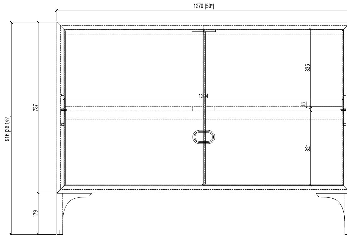
FRONT VIEW
