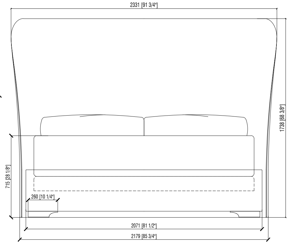
FRONT VIEW
