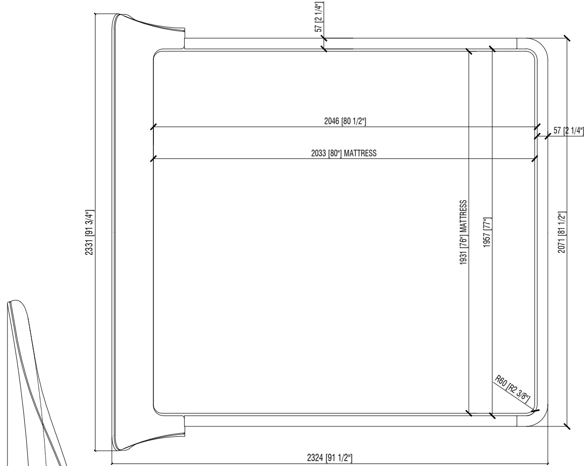
PLAN VIEW
