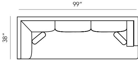
RIGHT ARM FACING LEFT CORNER SOFA 609-54 W 99 x D 38 x H 35 in
